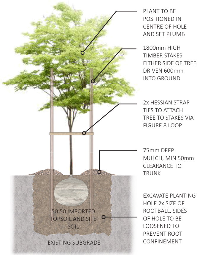
ON GRADE TREE DETAIL NTS
