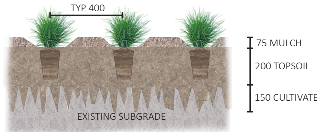
TYPICAL 200mm POT DETAIL NTS
