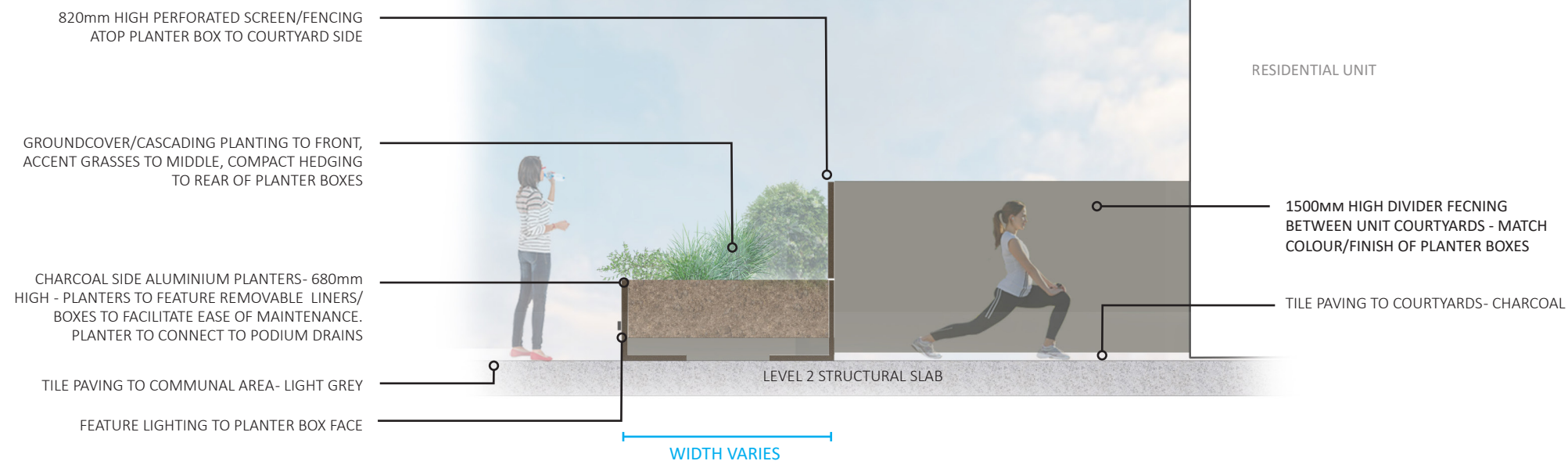
SECTION C - LEVEL 2 COURTYARD-COMMUNAL INTERFACE
