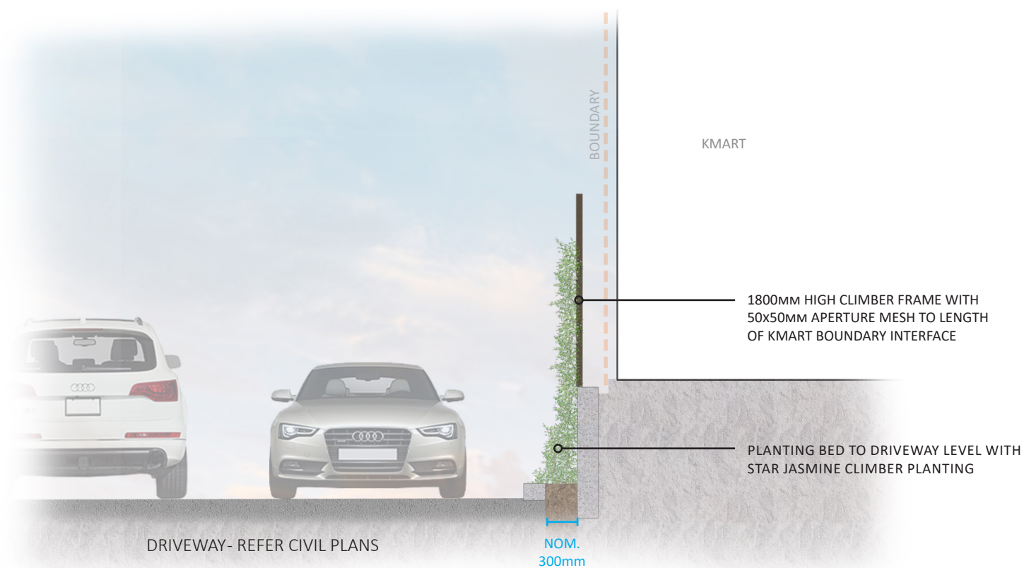
SECTION D - KMART BOUNDARY INTERFACE
